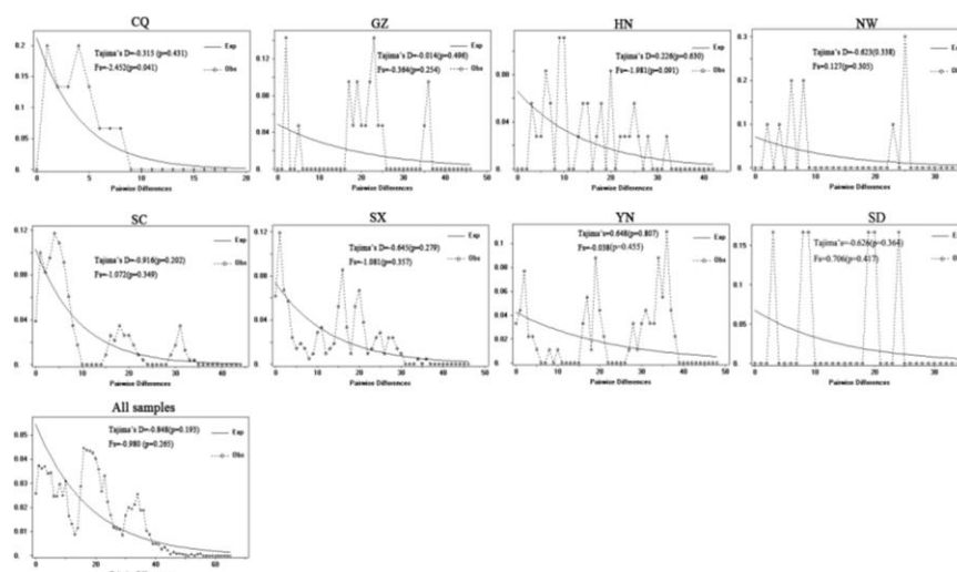
Fig. 2: The population demography analysis for A. Carmichaelii
