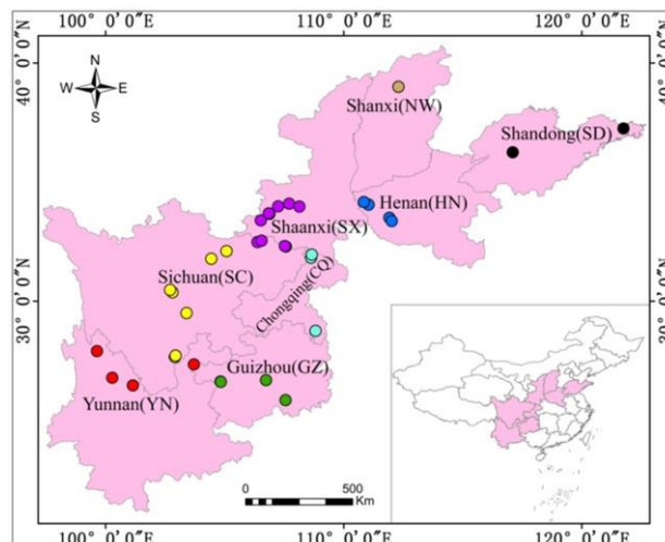
Fig. 1: The distribution of A. carmichaelii samples used in this study
