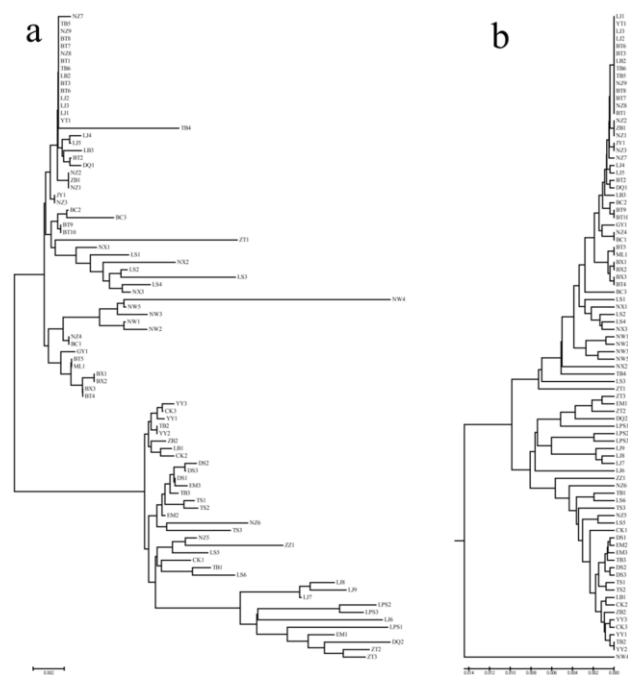
Fig. S1: NJ tree (a) and UPGMA tree (b) of A. carmichaelii samples
