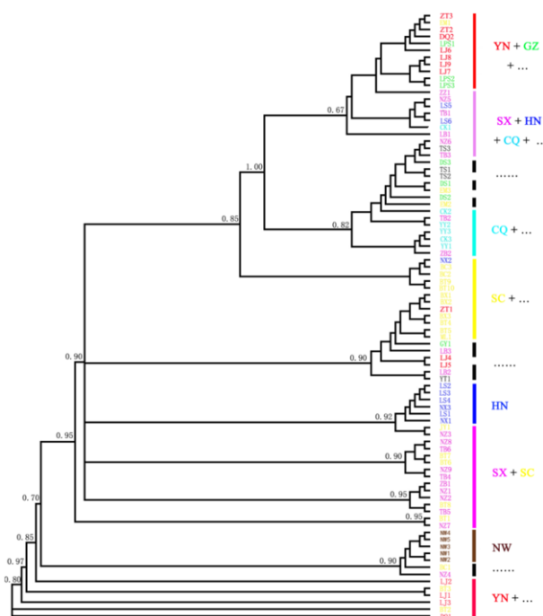
Fig. 3: Phylogenetic tree of A. Carmichaelii constructed with Bayesian inference. Numbers at nodes represent Bayesian posterior probabilities
