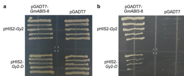
Fig. 5: The growth of yeast co-transformed with different vectors. (a) Control group. Culture medium without Trp and Leu. Sections 1 to 4 contain pGADT7- GmABI3-8 and pHis2- Gy2 , pGADT7 and pHis2- Gy2 , pGADT7- GmABI3-8 and pHis2- Gy2-D , and pGADT7 and pHis2- Gy2-D , respectively. (b) Treatment group. Culture medium without Trp, Leu and His. Sections 1 to 4 contain pGADT7- GmABI3-8 and pHis2- Gy2 , pGADT7 and pHis2- Gy2 , pGADT7- GmABI3-8 and pHis2- Gy2-D , and pGADT7 and pHis2- Gy2-D , respectively
