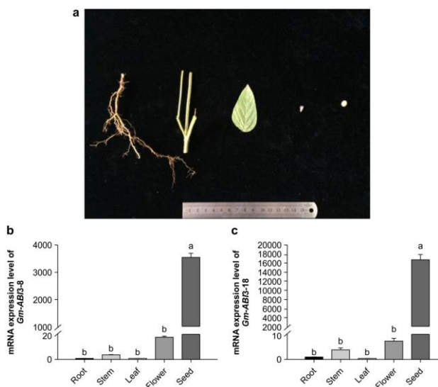
Fig. 1: The mRNA expression pattern of GmABI3-8 and GmABI3-18 in different plant tissues at 40 d post flowering. (a) From left to right: soybean root, stem, leaf, flower, and seed. (b) The mRNA expression pattern of GmABI3-8 . (c) The mRNA expression pattern of GmABI3-18 . Each value is the average of three datasets. Standard error is denoted by error bars. Means followed by the different letters within an accession are significantly different at P < 0.05
