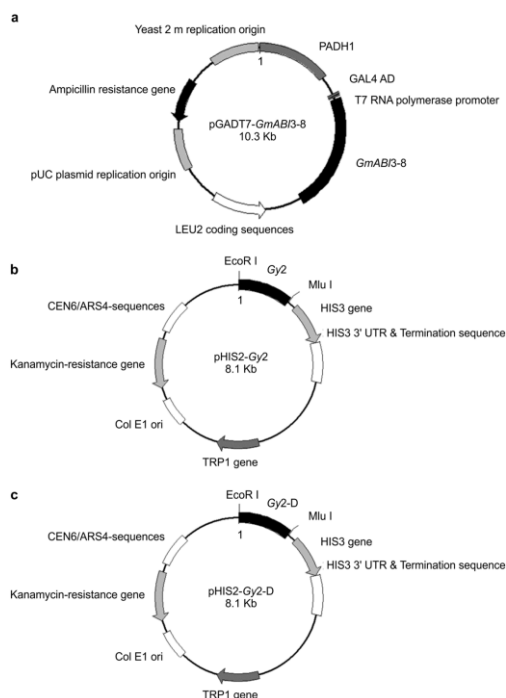
Fig. 4: Vectors used in the yeast one-hybrid system. (a) pGADT7- GmABI3-8 vector. (b) pHIS2- Gy2 vector. (c) pHIS2- Gy2-D vector
