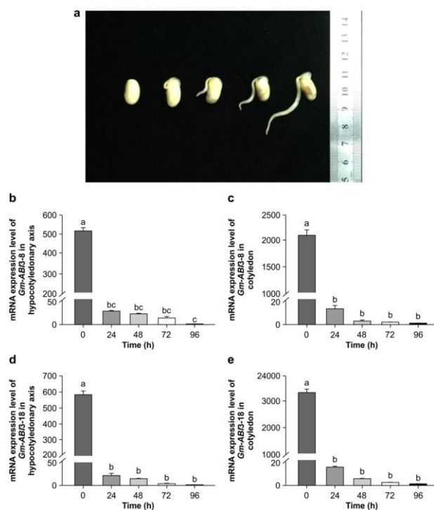
Fig. 2: The mRNA expression pattern of GmABI3-8 and GmABI3-18 in hypocotyledonary axis and cotyledon during seed germination. (a) Hypocotyledonary axis and cotyledon at 0 h, 24 h, 48 h, 72 h, and 96 h post imbibition for 6h. (b) The mRNA expression pattern of GmABI3-8 in the hypocotyledonary axis. (c) The mRNA expression pattern of GmABI3-8 in the cotyledon. (d) The mRNA expression pattern of GmABI3-18 mRNA in the hypocotyledonary axis. (e) The mRNA expression pattern of GmABI3-18 mRNA in the cotyledon. Each value is the average of three datasets. Standard error is denoted by error bars. Means followed by the different letters within an accession are significantly different at P < 0.05
