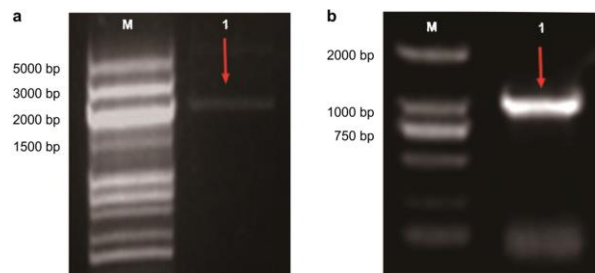
Fig. 3: Agarose gel electrophoresis of GmABI3-8 and Gy2 promoter. (a) Agarose gel electrophoresis of GmABI3-8 . Lane M is a 5,000 bp DNA marker. Lane 1 is GmABI3-8 . (b) Agarose gel electrophoresis of Gy2 promoter. Lane M is a 2,000 bp DNA marker. Lane 1 is the Gy2 promoter
