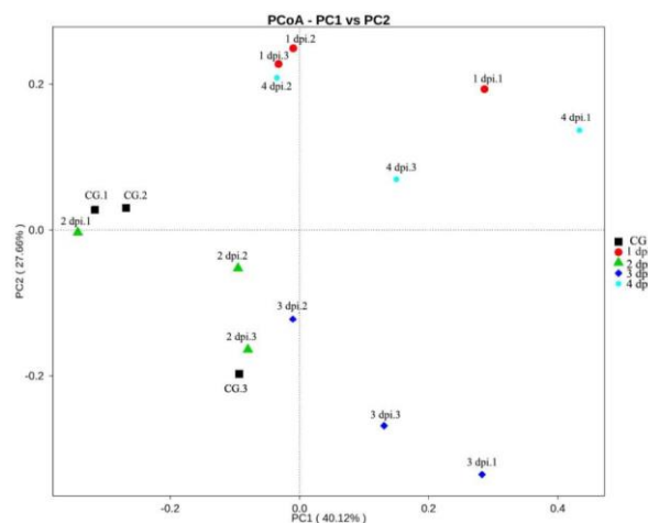
Fig. 4: Two-dimensional principal coordinates analysis (PCoA) plot of weighted unifracs distance matrices for intestinal microflora of Cynoglossus semilaevis . The percentage of variation indicated by the principal coordinates is shown on the axes; Black, red, green, dark blue and blue represent samples of CG, 1 dpi, 2 dpi, 3 dpi and 4 dpi, respectively; The samples of CG and 2 dpi, the samples of 1 dpi and 4 dpi and the samples of 3 dpi were respectively grouped into three distinct clusters
