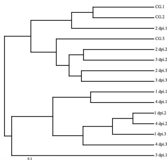
Fig. 5: Hierarchical clustering of microbiota from intestine of Cynoglossus semilaevis . Samples of 1 dpi and 4 dpi formed a distinct cluster, while the samples of CG and 2 dpi were more similar
