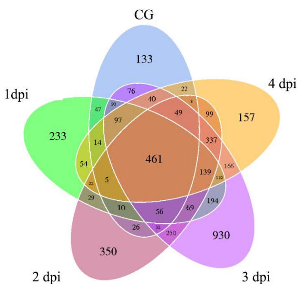
Fig. 1: Venn Diagram of OTUs from all the groups. Total 4308 OTUs were identified in 5 group; 1169, 1633, 1942, 3099, 1780 OTUs were found in CG, 1 dpi, 2 dpi, 3 dpi and 4 dpi, respectively; 461 OTUs were shared by all groups and 133, 233, 350, 930 and 157 were unique in CG, 1 dpi, 2 dpi, 3 dpi and 4 dpi, respectively
