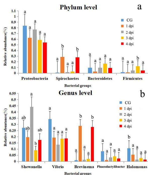
Fig. 2: Relative abundance of the dominant bacteria in the intestine of Cynoglossus semilaevis . (a): At phylum level, Proteobacteria, Spirochaetes, Bacteroidetes and Firmicutes were the dominant phyla in all groups; (b): At genus level, Shewanella , Vibrio , Brevinema , Phaeodactylibacter , Halomonas were identified as the major bacterial taxa in all groups. The difference letters on the bar chart indicated significant difference among the different groups at P < 0.05 level
