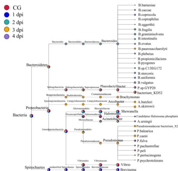
Fig. 3: Species taxonomy tree was structured on a basic of genera with top 10 relative abundances. Total 31 species of Bacteroides , Phaeodactylibacter , Arcobacter , Halomonas , Acinetobacter and Pseudomonas were detected; Shewanella , Brachymonas , Vibrio , Brevinema were not identified to the species level
