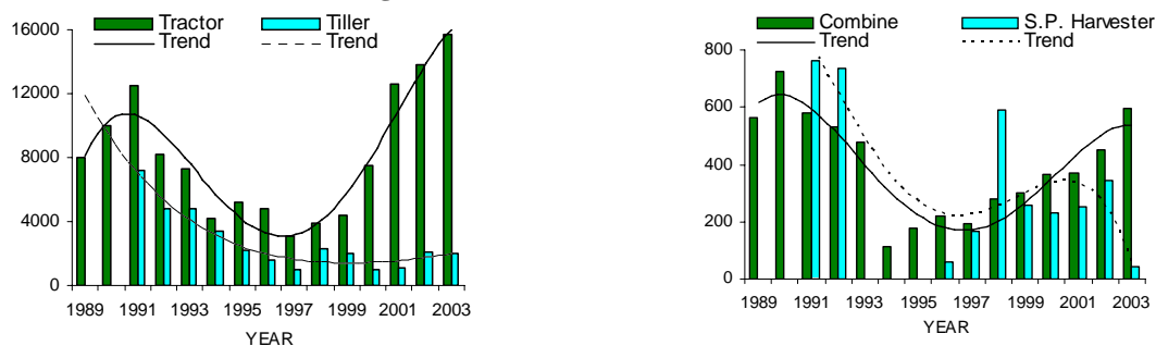
(a) Tractor and tiller
