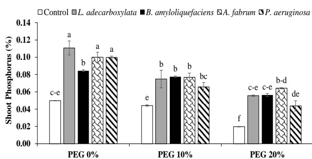
Fig. 3: Effect of ACC deaminase containing PGPRs on wheat shoot phosphorus concentration under osmotic stress \pm SE. Means sharing the same letter are statistically similar p \leq 0.01
